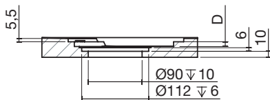
SECTION C
